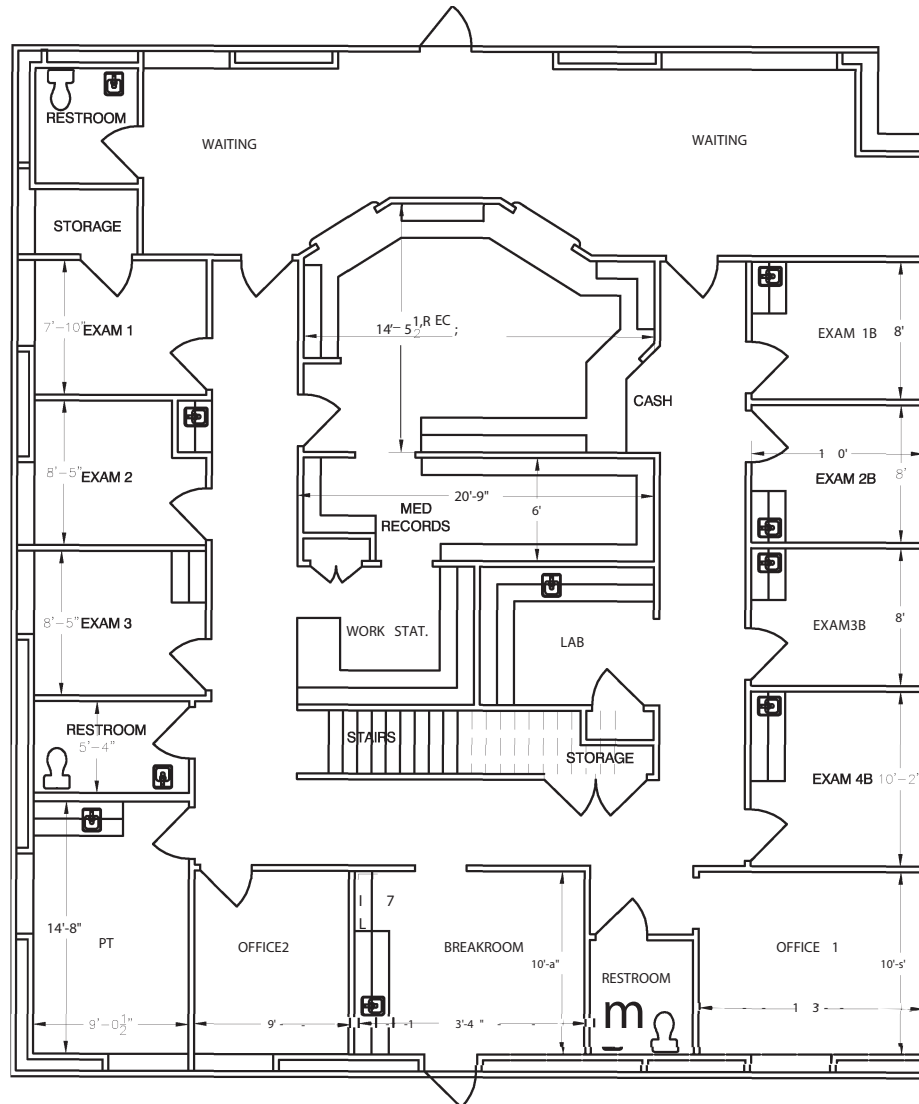
MAIN LEVEL
