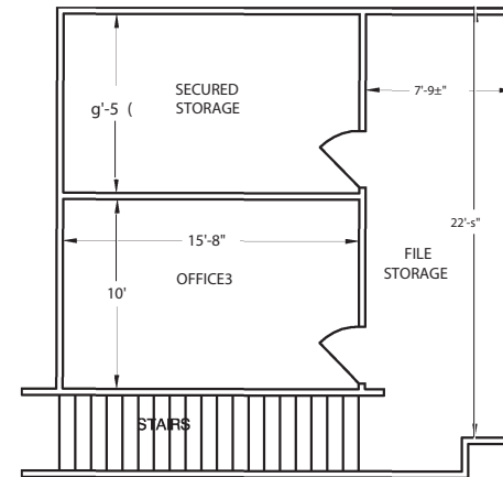
MEZZANINE
